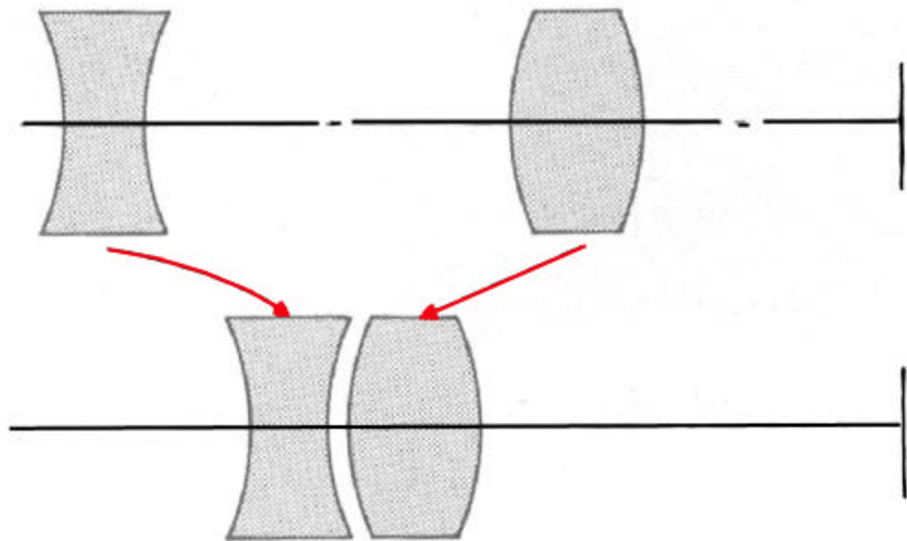
2-group zooming
