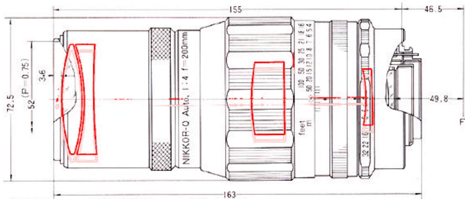
200mm f/4 Nikkor-Q Auto
